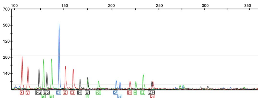
Fig. 1. An electropherogram (epg) showing several peaks close to the reporting threshold of 50 RFU (lower grey line). The highest peak, labelled 13, has no partner but since it is above the LTDNA threshold of 300 RFU (upper grey line) it is assumed to represent a 13,13 homozygote. In contrast, the genotypic designation 11,0 for a low peak allows the possibility of any other allele, including another 11, in the genotype of the contributor.
