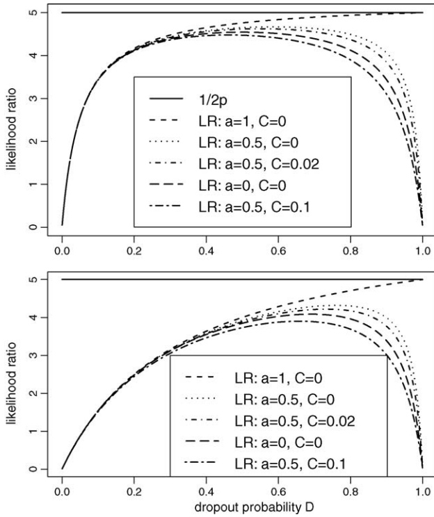
Fig. 2. Single-locus likelihood ratios ( LR ) when CSP \equiv A and s \equiv AB , without masking (top, Eq. (1)) and when there are two masking alleles (bottom, Eq. (2)). The locus is assumed to have ten equally frequent alleles (no F_{ST} or sampling adjustment), and \alpha (a in legend box) is defined by D_2 = \alpha D^2 , where D_2 denotes the homozygote drop-out probability. The drop-in probability is denoted C .
