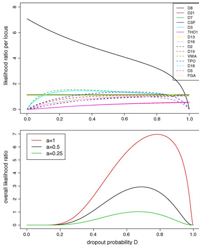
Fig. 6. Top. Single locus LR s as a function of D for the CSP of Table 3, using \alpha = 0.5 and C = 0.05 and F_{ST} = 0.02 . CSP alleles that are attributable to \nu are assumed to be masking. Bottom. Black curve: whole profile LR (=product of single-locus LR s). Red and green curves show the effect of varying the homozygote drop-out parameter \alpha (see text for discussion).
