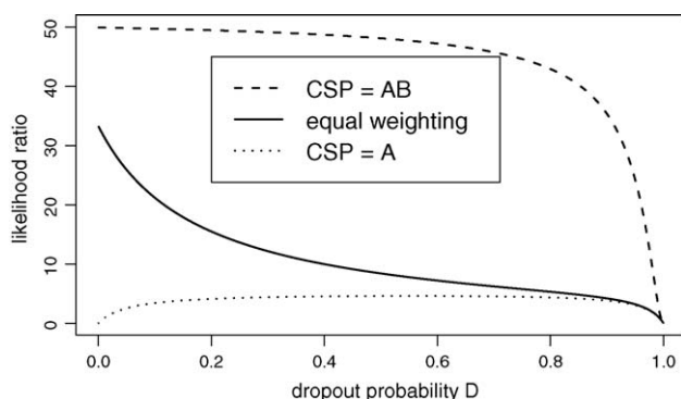
Fig. 4. Single locus LR s as a function of D for a single-contributor profile for which the alleged contributor has genotype AB . Dashed curve: CSP is called as AB ; dotted curve: CSP is called as A ; solid curve: LR obtained by averaging both numerator and denominator over the two possible calls corresponding to certainty about allele A but only a 0.5 probability that the unknown contributor has allele B . We use \alpha = 0.5 and C = 0.02 ; other details as for Fig. 2.
