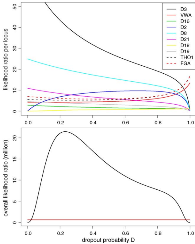
Fig. 5. Top. Single-locus LRs as a function of single-allele drop-out probability D , for the CSP of Table 1, using \alpha = 0.5 and C = 0.05 and F_{ST} = 0.02 . Bottom. Black curve: whole profile LR (=product of single-locus LRs). Red line: RMNE value reported in court.
