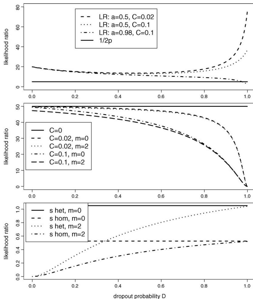
Fig. 3. Top: Single-locus LRs when CSP \equiv A and s \equiv AA and there are two masking alleles. Middle: Single-locus LRs when CSP \equiv AB and s \equiv AB , without masking ( m = 0 ) and when there are two masking alleles ( m = 2 ). Bottom: Single-locus LRs for a null CSP, with and without masking, in each case with \alpha = 0.5 and C = 0.02 . Other details as for Fig. 2. When m = 0 the LR is constant, 1.053 when s is heterozygous, and 0.546 when s is homozygous.
