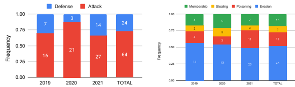
(a) G1: What is the focus of the paper? (b) G2: What is the main attack family ?
